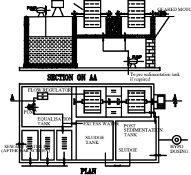
SEWAGE TREATMENT PLANT DETAILS
