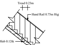
STAIR DETAILS SCALE : 1:50
