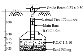
FOOTING DETAILS SCALE : NOT TO SCALE
