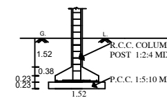
COLUMN POST DETAILS
