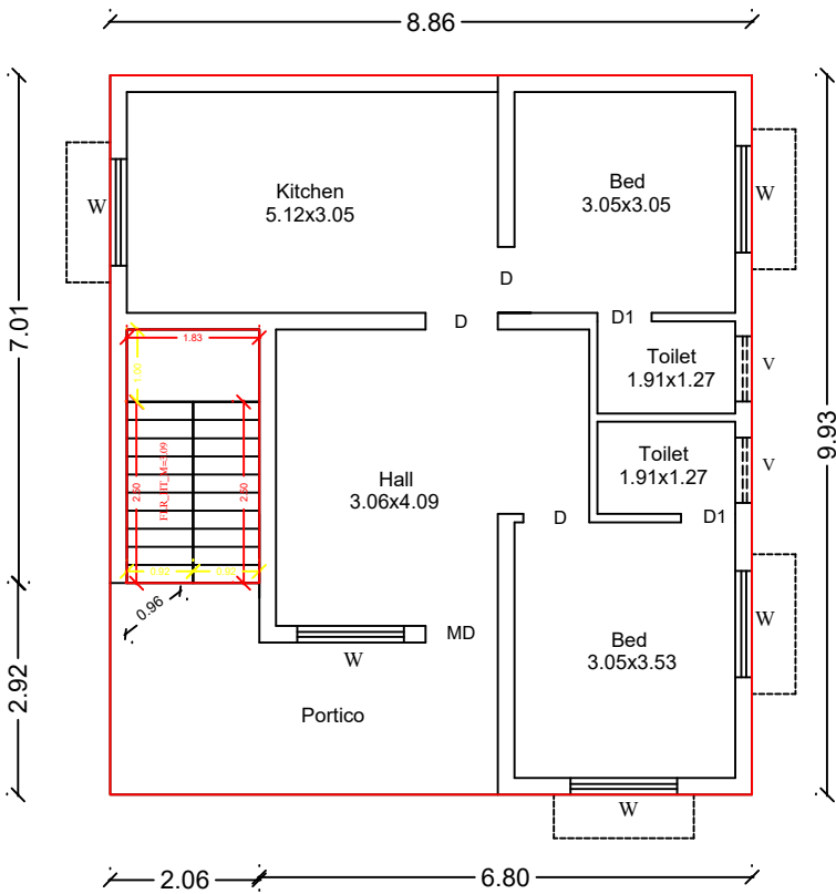
Ex GROUND FLOOR PLAN
