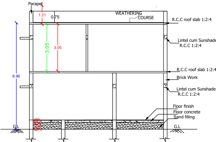
SECTION ON "A S"
