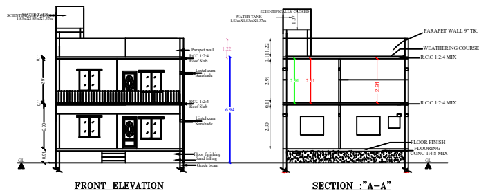
FRONT ELEVATION
