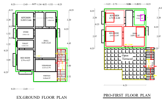
EX-GROUND FLOOR PLAN
