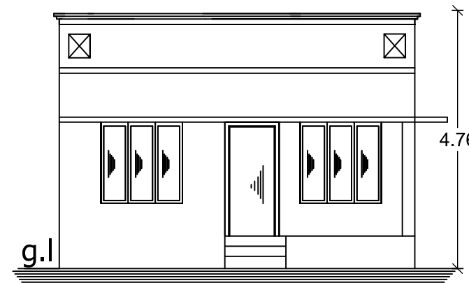
Building Front Elevation
