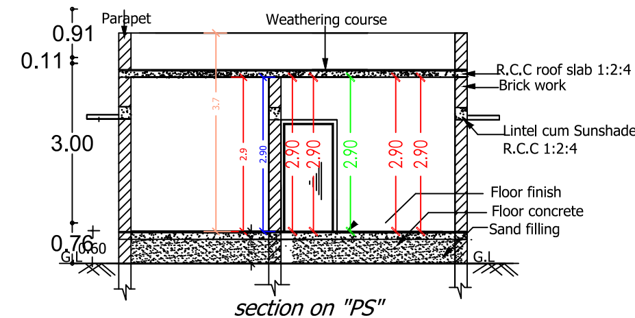
section on "PS"
