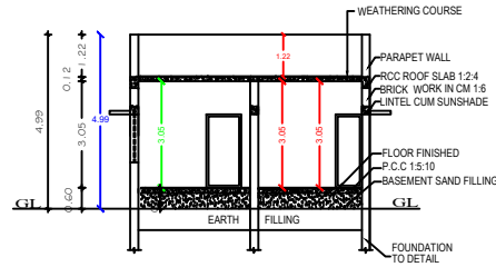
SECTION "A-B"
