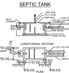
SEPTIC TANK
