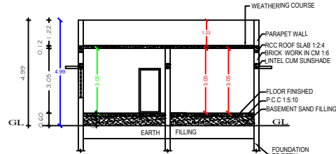
SECTION "A-B"
