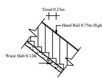
STAIR DETAILS SCALE : 1:50
