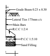
DETAILS NOT TO SCALE
