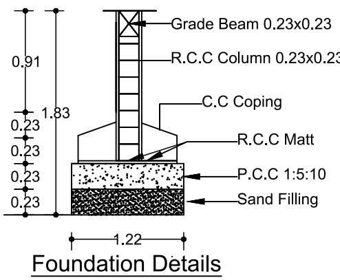
Foundation Details
