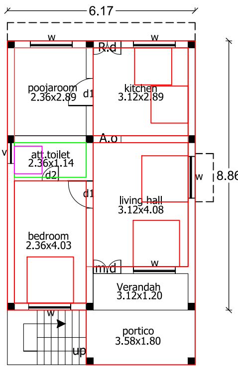
Proposed g.f Building plan
