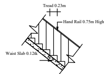
STAIR DETAILS SCALE : 1:50
