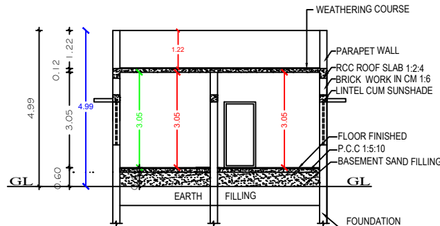
SECTION "A-B"
