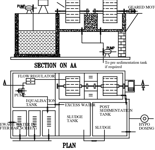
SEWAGE TREATMENT PLANT DETAILS
