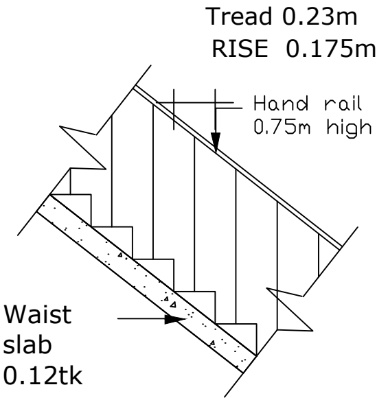
STAIRCASE
