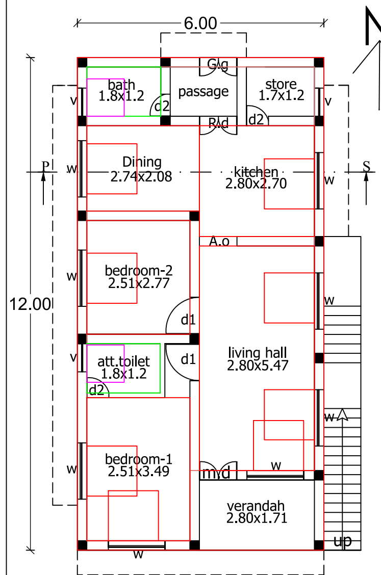
Proposed g.f Building plan
