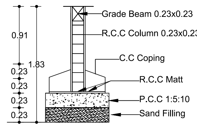
Foundation Details
