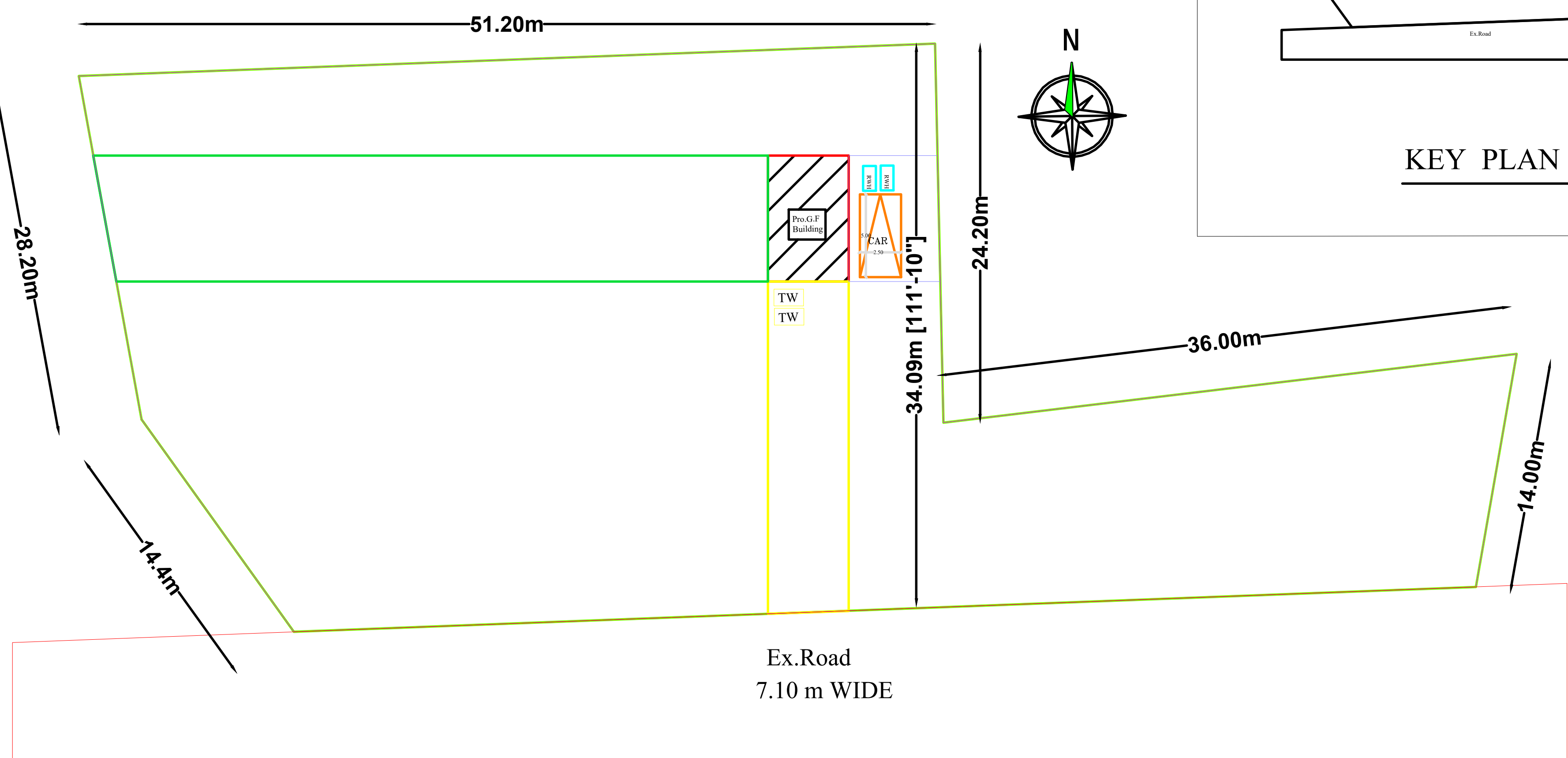
SITE PLAN
