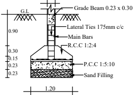
FOOTING DETAILS SCALE : NOT TO SCALE
