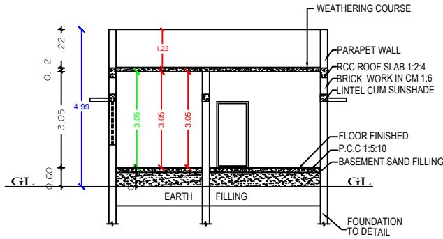
SECTION ON "J-J"
