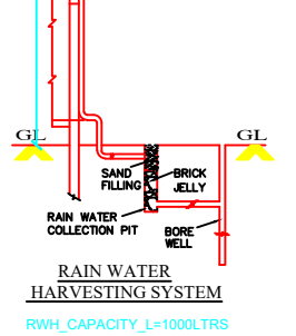
RAIN WATER HARVESTING SYSTEM RWV_CAPACITY_L=1000LTRS
