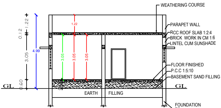
SECTION ON "J-J"
