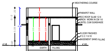
SECTION ON "J-J"
