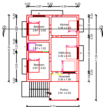
PRO.GROUND FLOOR PLAN
