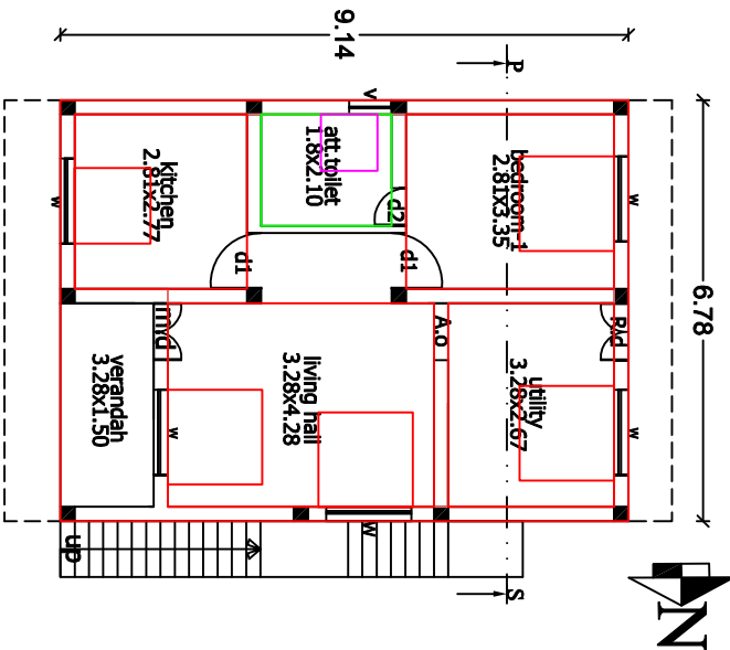
Proposed g.f Building plan
