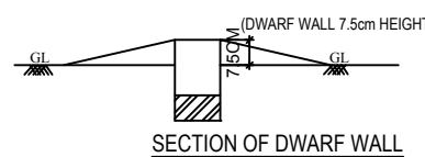
COMPOUND WALL DETAIL SCALE - 1 : 50
