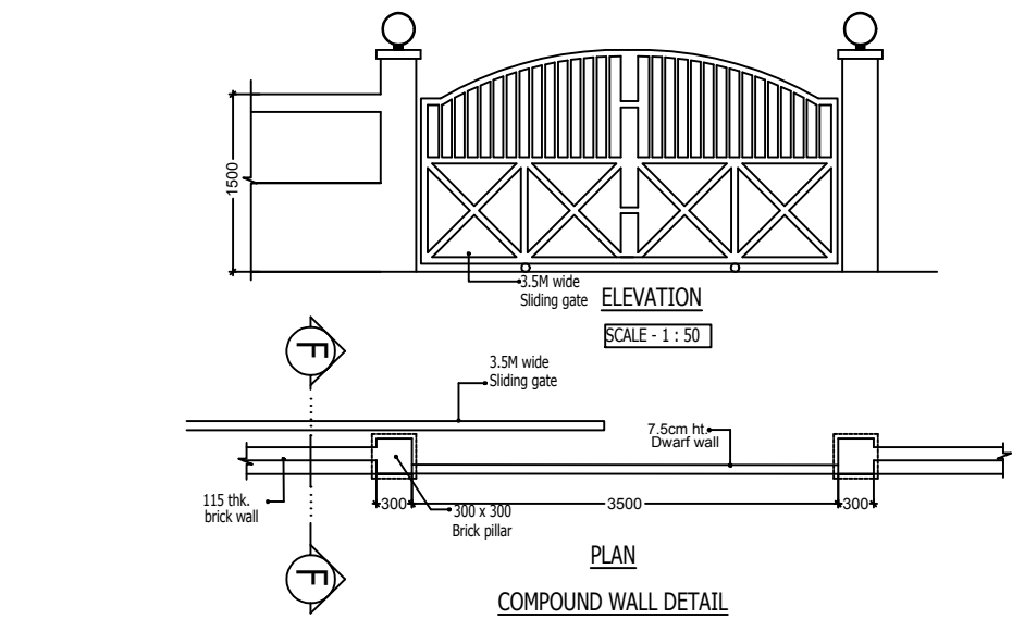
COMPOUND WALL DETAIL SCALE - 1 : 50
