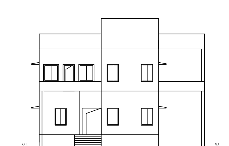
FRONT ELEVATION
