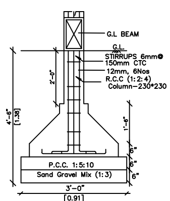
R.C.C. COLUMN FOOTING DETAILS SCALE : 1:25
