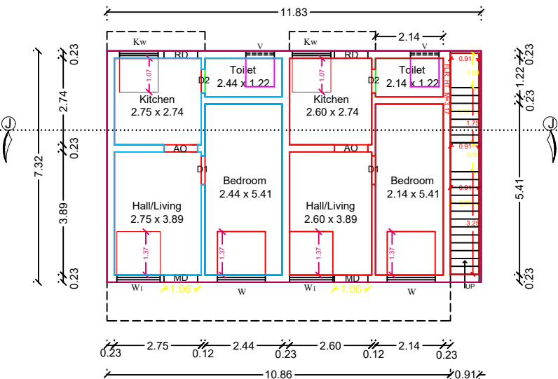
PRO.GROUND FLOOR PLAN
