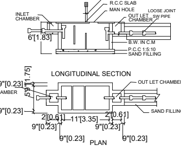
SEPTIC TANK
