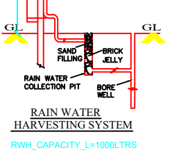
PERCULATION PIT
