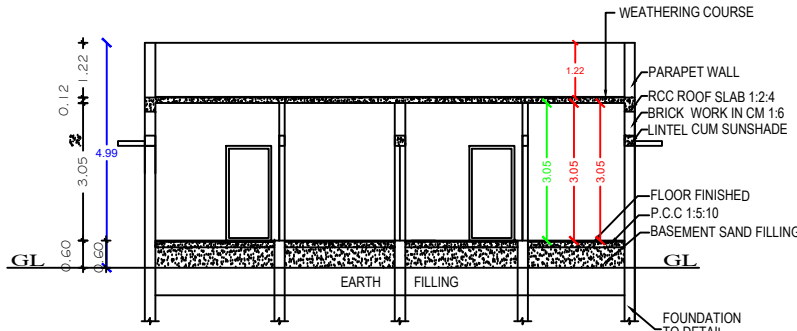
SECTION ON "J-J"
