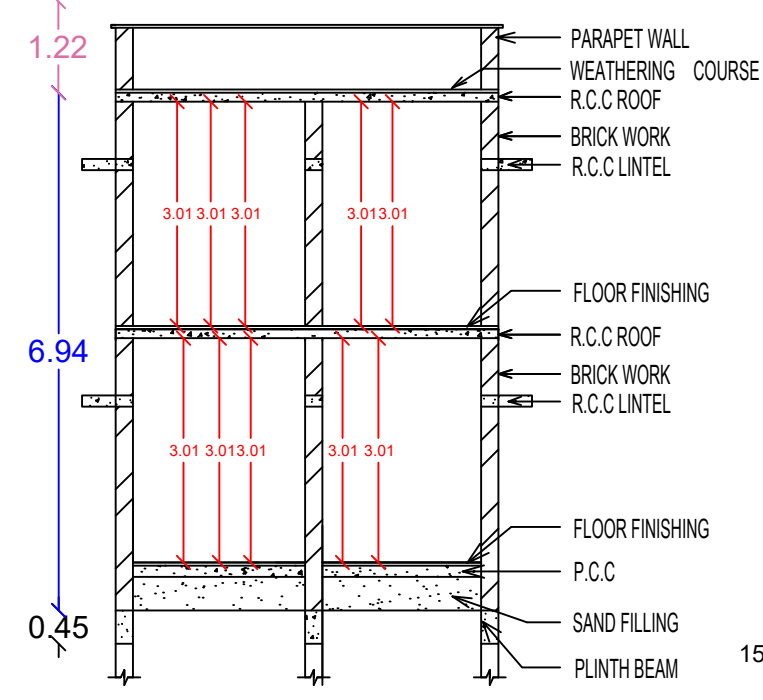
SECTION ON R-S
