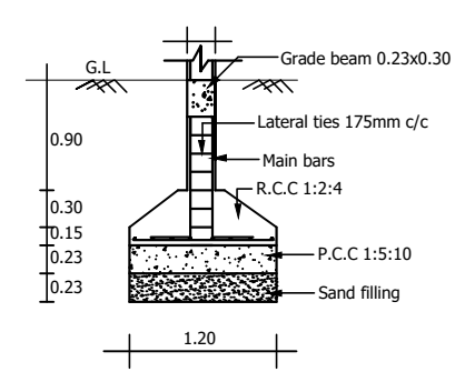
FOOTING DETAILS NOT TO SCALE
