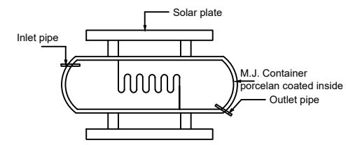
SOLAR WATER HEATING SYSTEM SCALE:NOT TO SCALE
