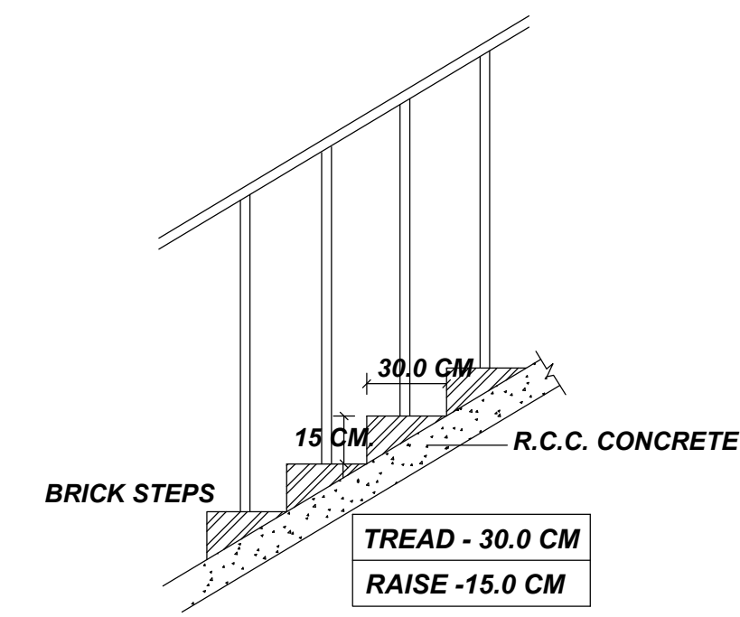
STAIRCASE DETAILS NTS
