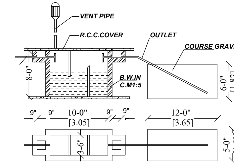
SEPTIC TANK & D-TRENCH DETAILS (NOT TO SCALE)
