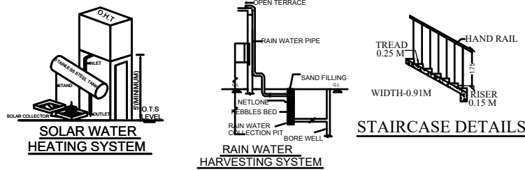
RAIN WATER HARVESTING SYSTEM
