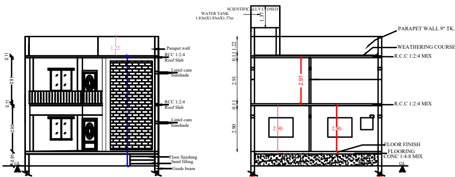
FRONT ELEVATION
