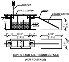
SEPTIC TANK & D-TRENCH DETAILS (NOT TO SCALE)
