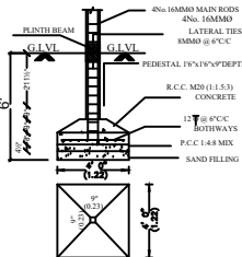
FOUNDATION DETAIL (SCALE 1:10)
