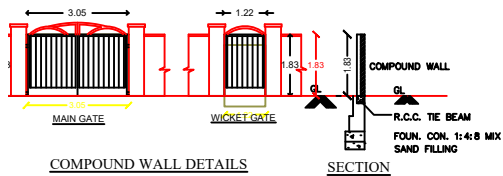
COMPOUND WALL DETAILS
