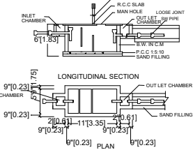
SEPTIC TANK
