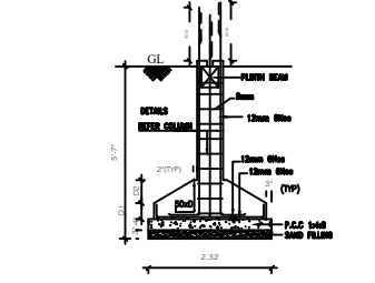
FOUNDATION DETAILS SCALE : 1:50.
