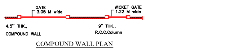
COMPOUND WALL PLAN
