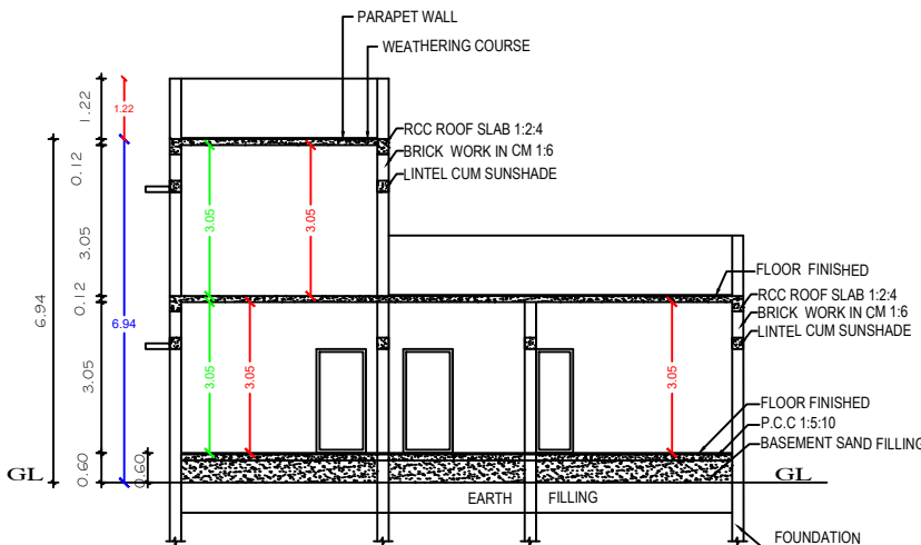
SECTION "J-J"
