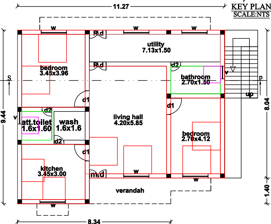
Proposed ground floor Building plan
