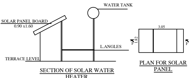
SECTION OF SOLAR WATER HEATER
