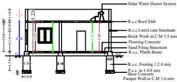
SECTION ON - "XX"
