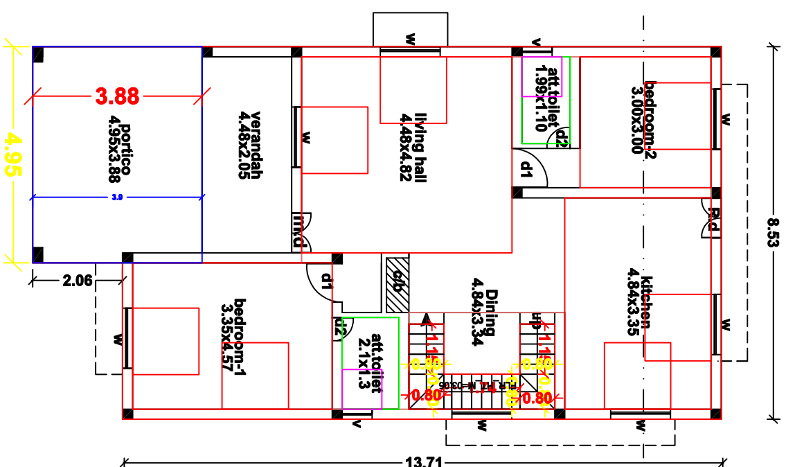
Proposed g.f Building plan
