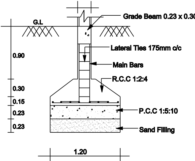
FOOTING DETAILS SCALE : NOT TO SCALE
