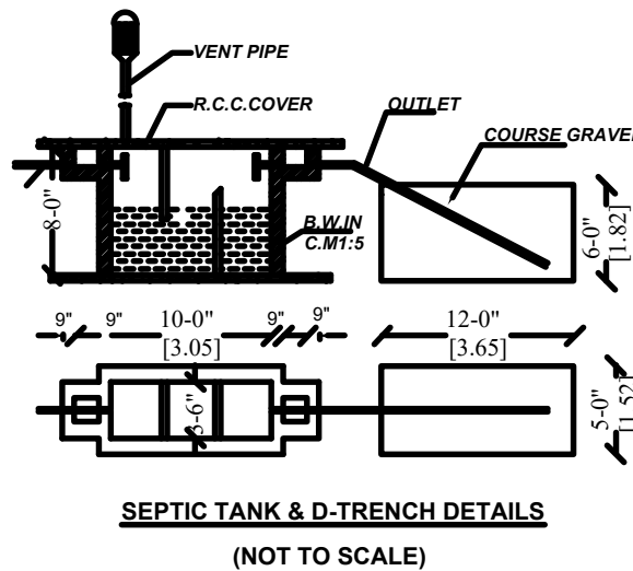
SEPTIC TANK & D.T. TRENCH DETAILS (NOT TO SCALE)
