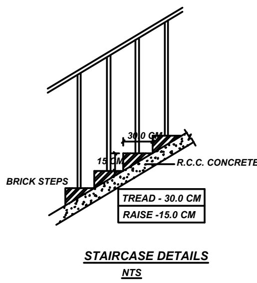
STAIRCASE DETAILS SITE
