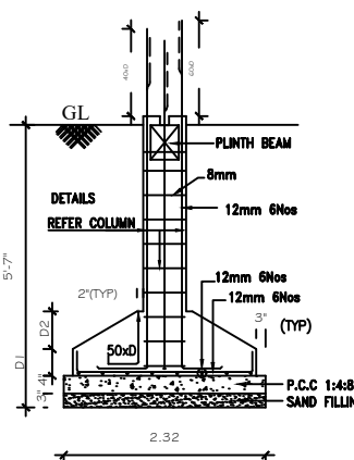
FOUNDATION DETAILS SCALE : 1:50.
