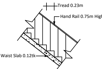
STAIR DETAILS SCALE : 1:50
