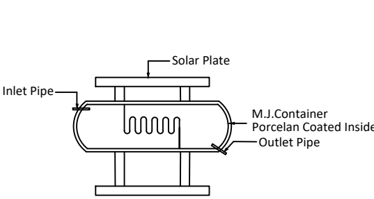
SOLAR WATER HEATING SYSTEM SCALE : NOT TO SCALE
