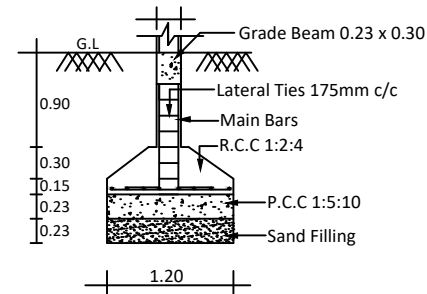
FOOTING DETAILS SCALE : NOT TO SCALE
