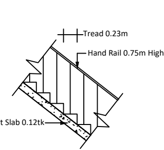
STAIR DETAILS SCALE : 1:50
