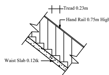
STAIR DETAILS SCALE : 1:50
