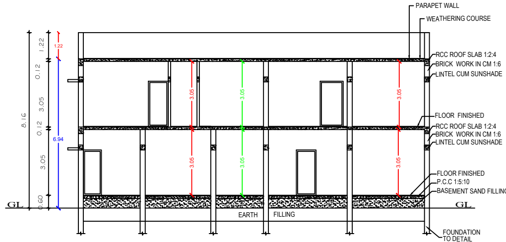
SECTION "J-J"
