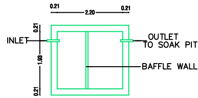
PLAN SEPTIC.TANK
