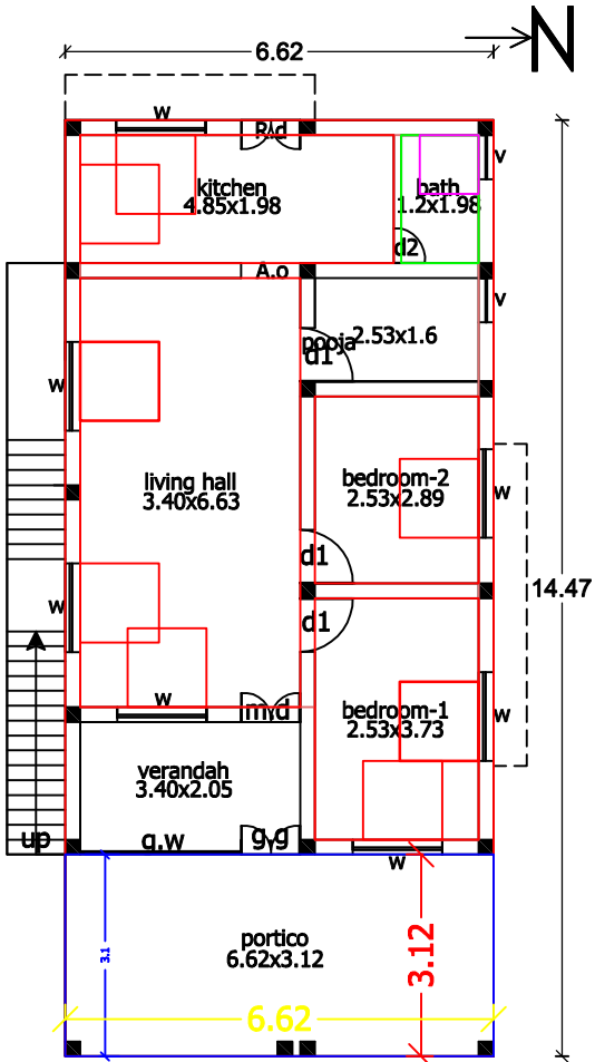
Proposed g.f Building plan
