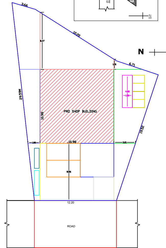
SITE PLAN
