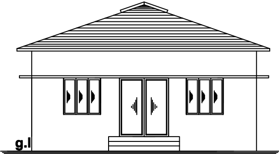
Building Front Elevation
