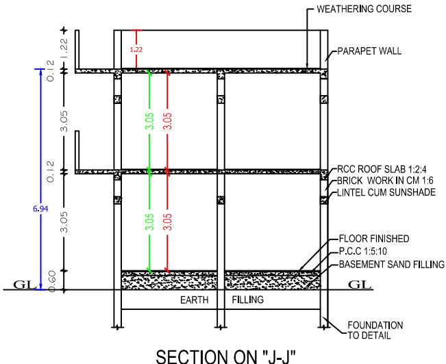
SECTION ON "J-J"
