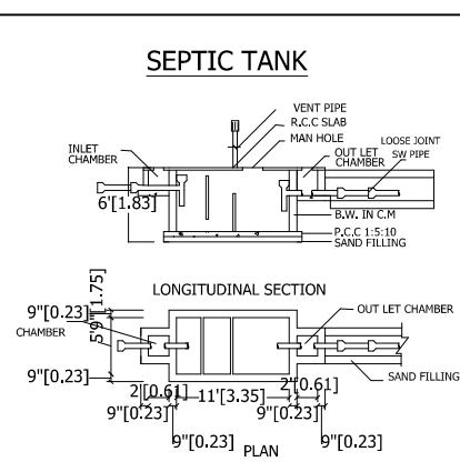
SEPTIC TANK
