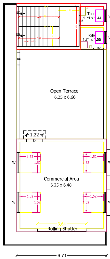
PROPOSED FIRST FLOOR PLAN
