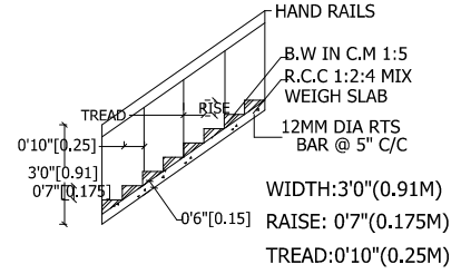
FOUNDATION DETAILS
