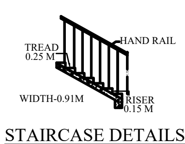
STAIRCASE DETAILS
