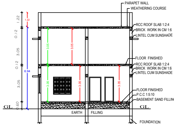
SECTION "J-J"
