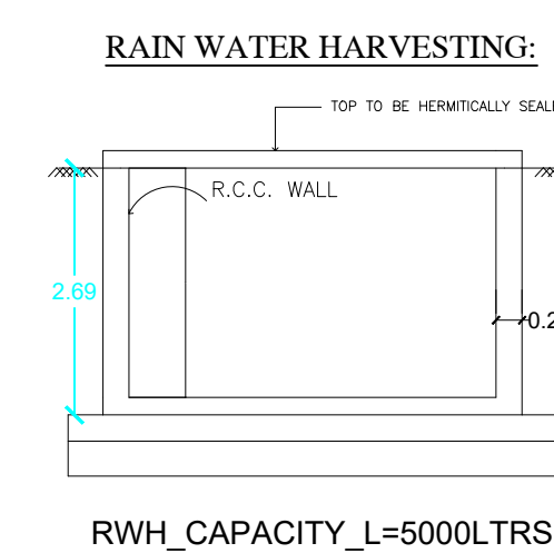
RWH_CAPACITY_L=5000LTRS
