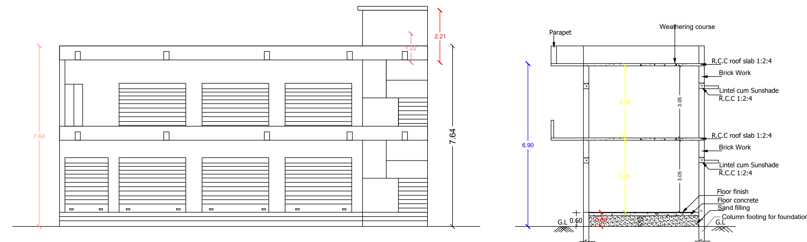
SECTION ON "A S"
