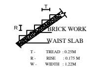
STAIRCASE DETAILS (NOT TO SCALE)
